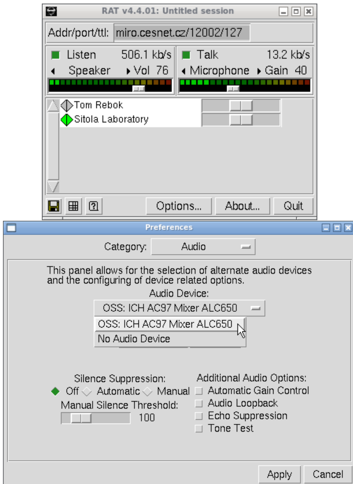
Figure 1. The main screen and audio devices' selection screen of the original RAT.
