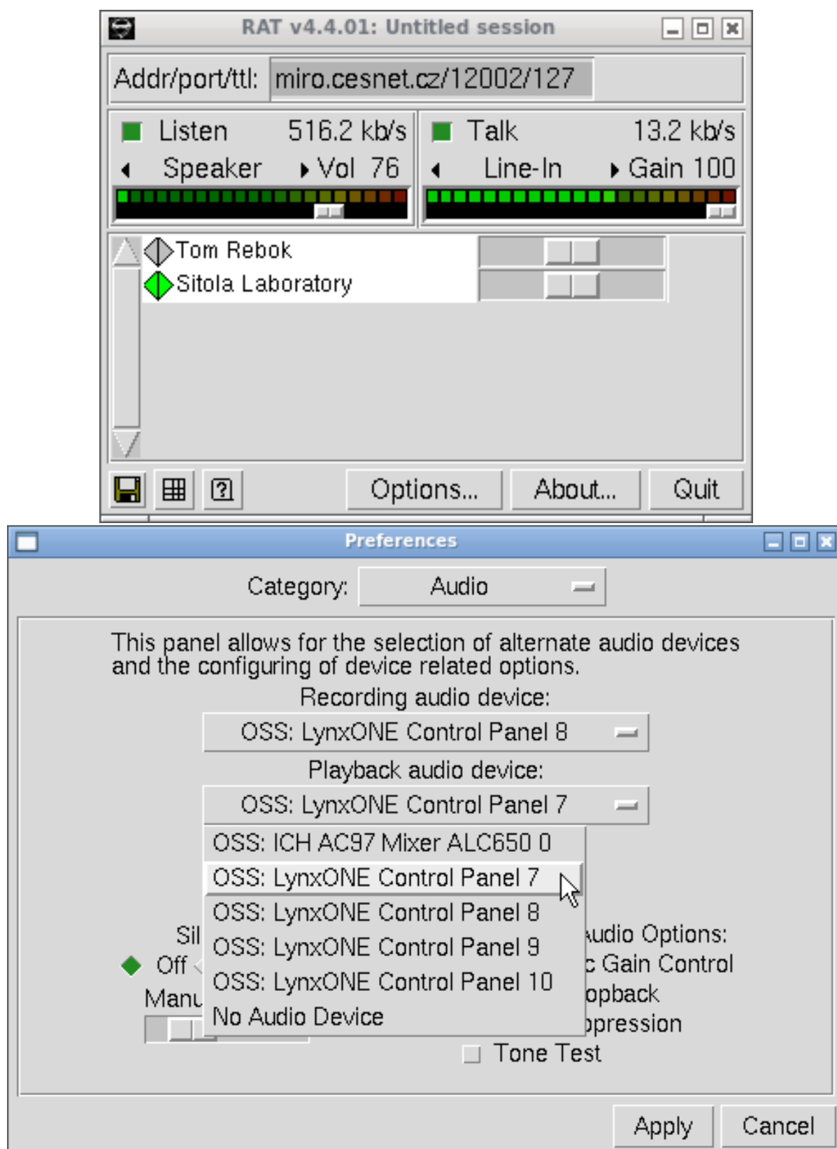
Figure 2. The main screen and audio devices' selection screen of RAT-HD.
